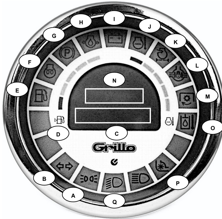
FIG.3 – DASHBOARD FIG.3 – CRUSCOTTO FIG.3 – TABLEAU DE BORD ABB.3 – ARMATURENBRETT FIG.3 – TABLERO DE CONTROL
